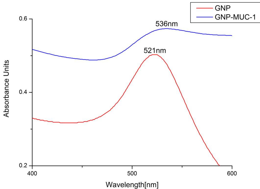
Figure S1. UV-Vis spectra of GNP (red line) and GNP-MUC-1 (blue line);
