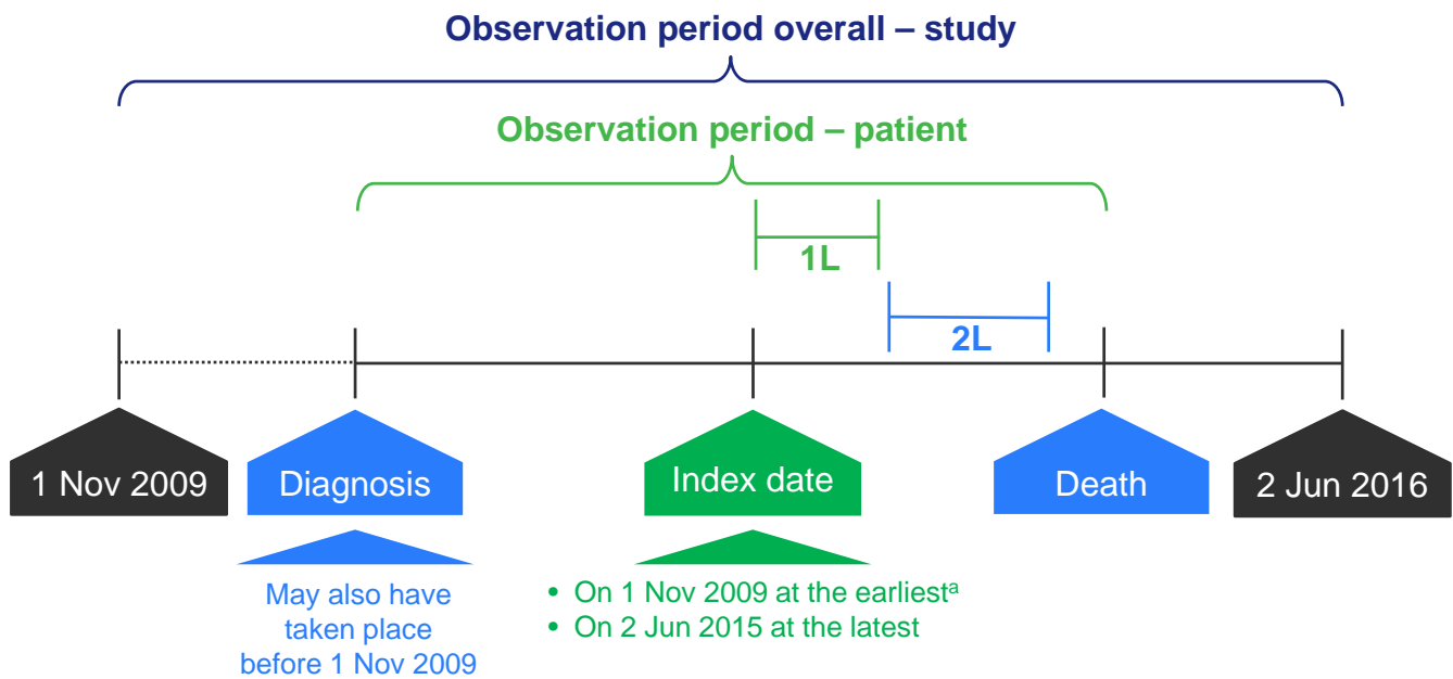
Figure S1. Study design. Schematic of the study periods relevant to analysis. a Patients may have received first-line (1L) treatment before 1 November 2009 and second-line (2L) treatment thereafter. Such patients were included in the analysis if data from both treatment settings were complete. For 1L treatment, the index date for study participants was the start date of the 1L systemic treatment. For 2L treatment, the index date was the date when the 2L chemotherapeutic treatment for recurrence after previous treatments/treatment failure of 1L treatment was initiated.
