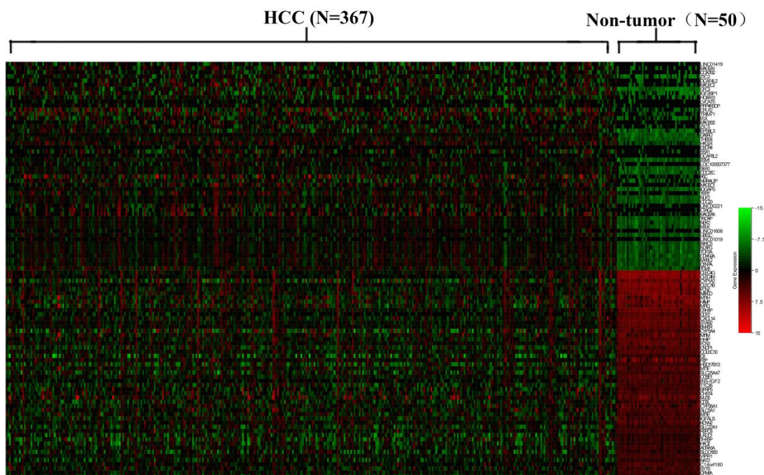
Supplementary Figure S2: The 100 top differential expressed mRNAs from TCGA RNAseq. The names of mRNA were shown on the right longitudinal axis; The information of samples was shown on the upper abscissa axis.
