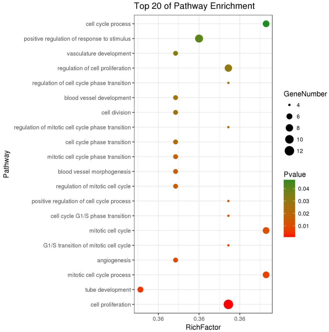
Supplementary Figure S4: The top 20 significant enriched GO term of differential mRNAs.
