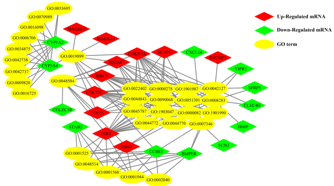
Supplementary Figure S3: The network of differential mRNAs and GO term annotation.
