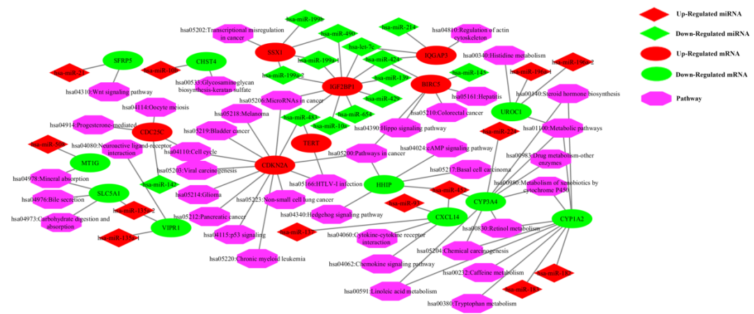
Supplementary Figure S5: The regulation network of mRNAs and pathways.
