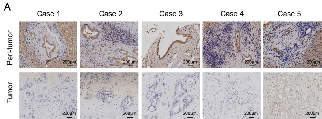
Figure S1. BLVRB depletion promoted cell migration by activating the Notch/Snail signaling pathway
