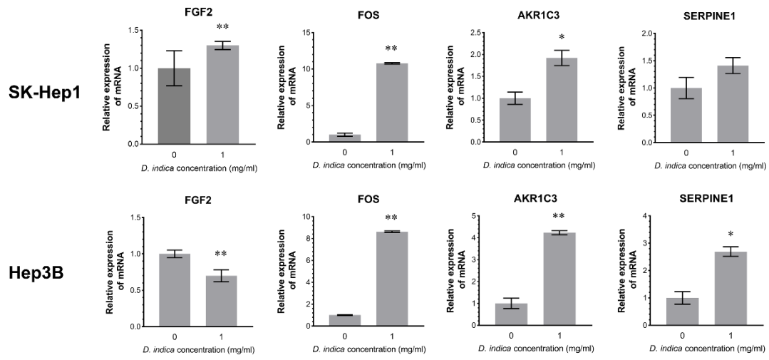
Figure S2. The expression levels of FOS, SERPINE1, AKR1C3, and FGF2 in SK-Hep1 and Hep3B cells with and without D. indica administration. *, p < 0.05 ; **, p < 0.01 .
