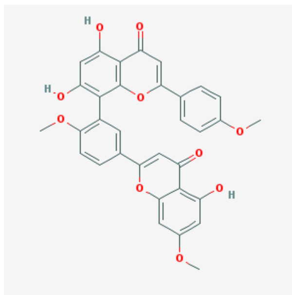
Figure S1. The molecular structure of sciadopitysin.
