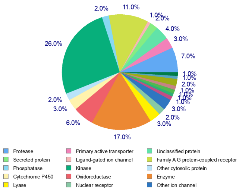
Figure S2. Classes of sciadopitysin potential targets.
