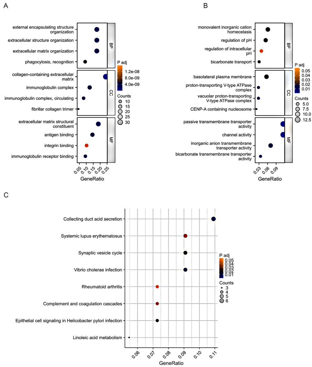
Figure S1. Enrichment analysis of the DEGs. (A and B) GO analysis of the DEGs. (C) KEGG analysis of the upregulated DEGs upon DOK1 knockdown.
